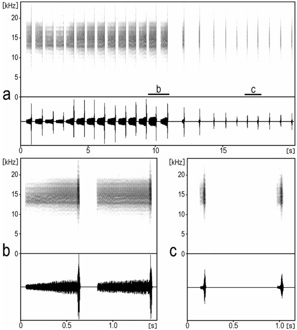
Fig. 3. Sonogram and oscillogram (a) of the end of the sequence of the calling song of Cicadetta cerdaniensis from Polana Polichno followed by the beginning of the next sequence; b) enlarged part of sonogram and oscillogram of double echeme (DE) from the end of the sequence with long low intensity part (LDE); c) enlarged part of sonogram and oscillogram of double echeme (DE) from the beginning of the sequence with short low intensity part (LDE). Since the microphone was not calibrated, there is no scale on oscillogram Y-axis (valid also for Fig. 4).
